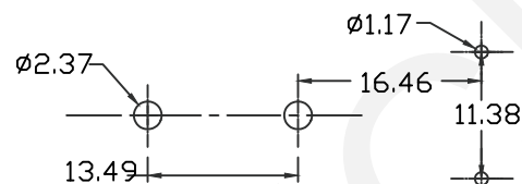
PCB LAYOUT
