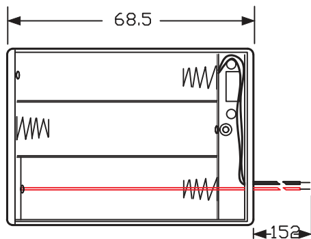
Holder
