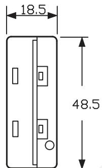
END VIEW
