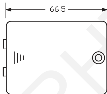
Cover
