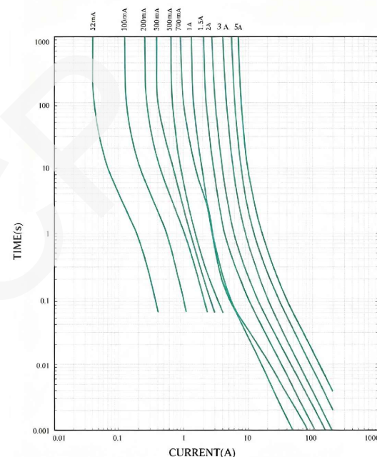
I-T CHARACTERISTICS CURVE
