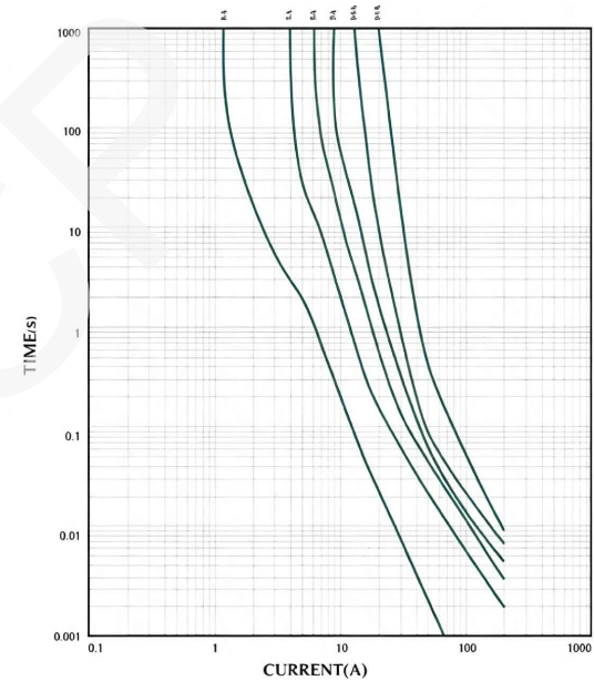
I-T CHARACTERISTICS CURVE
