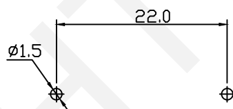
Mounting Holes
