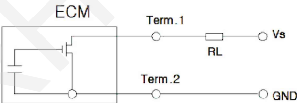
Schematic diagram VS=1.5V RL=680Ω
