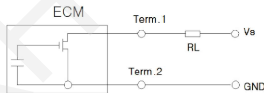
Schematic diagram VS=1.5V RL=680 \Omega
