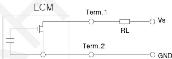
Schematic diagram VS=1.5V RL=680 \Omega
