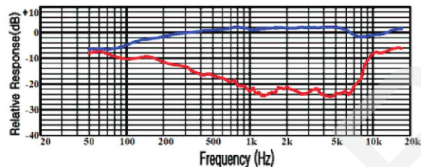
Frequency response
