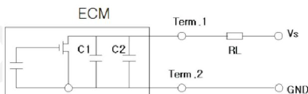
Schematic diagram VS=2V RL=2.2K
