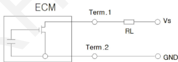
Schematic diagram VS=2V RL=2.2K
