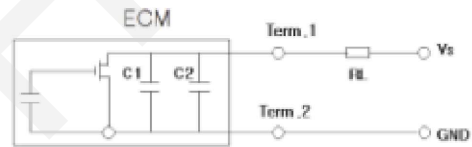
Schematic diagram VS=2V RL=2.2KΩ
