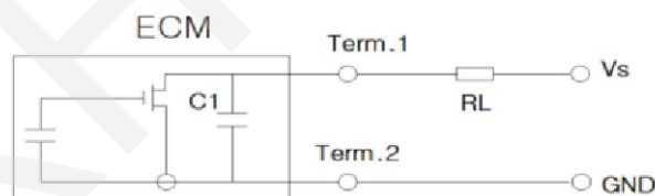
Schematic diagram VS=2V RL=2.2KΩ
