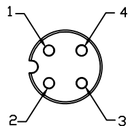
RHTDY12A-TR204PG9
