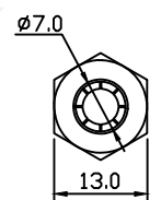
Cable outlet PG7
