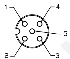
RHTDY12A-TR205PG7
