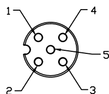
RHTDY12A-TR205PG9
