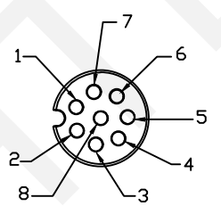
RHTDY12A-TR208PG7
