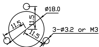
Panel mount
