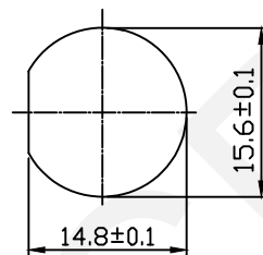
Panel Cut-out
