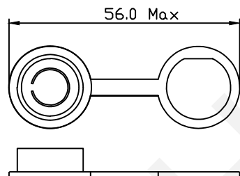
Protection cap for Male panel mount connector
