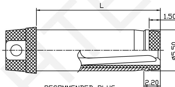
RECOMMENDED PLUG
