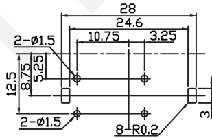
PCB HOLE LAYOUT(TOLERANCE:±0.1) BOTTOM VIEW
