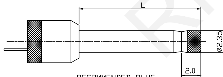
RECOMMENDED PLUG
