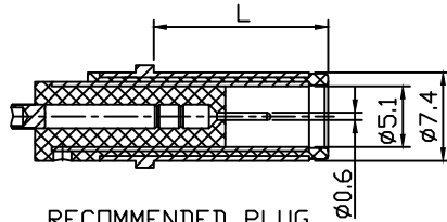
RECOMMENDED PLUG
