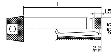
RECOMMENDED PLUG
