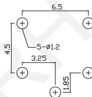
PCB LAYOUT
