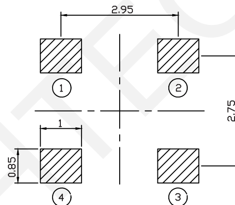
Installation diagram
