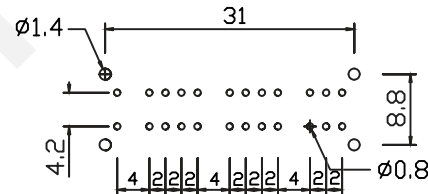
P.C.B.HOLE DETAIL
