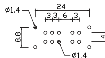
P.C.B.HOLE DETAIL
