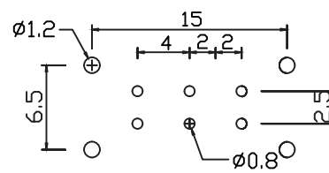
P.C.B.HOLE DETAIL
