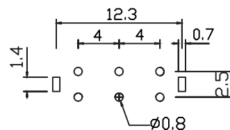
P.C.B.HOLE DETAIL
