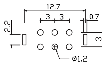
P.C.B.HOLE DETAIL
