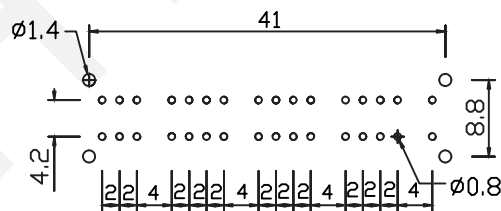
P.C.B.HOLE DETAIL
