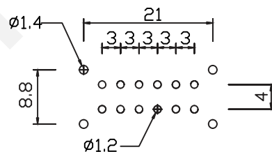
P.C.B.HOLE DETAIL
