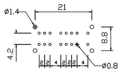
P.C.B.HOLE DETAIL
