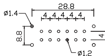
P.C.B.HOLE DETAIL
