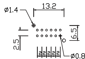
P.C.B.HOLE DETAIL
