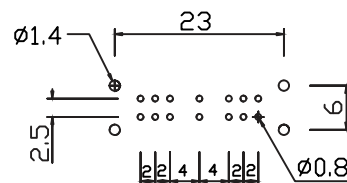
P.C.B.HOLE DETAIL
