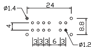
P.C.B.HOLE DETAIL
