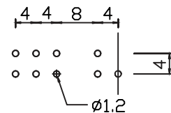
P.C.B.HOLE DETAIL
