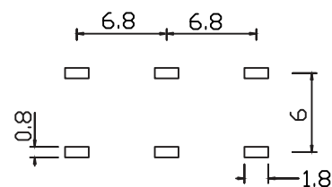
P.C.B.HOLE DETAIL
