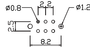
P.C.B.HOLE DETAIL
