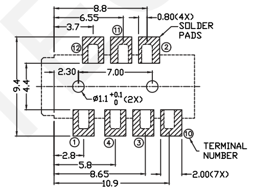
RECOMMENDED SOLDER PAD LAYOUT
