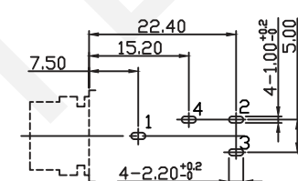
Pin Hole Layout (Jack Bottom View)
