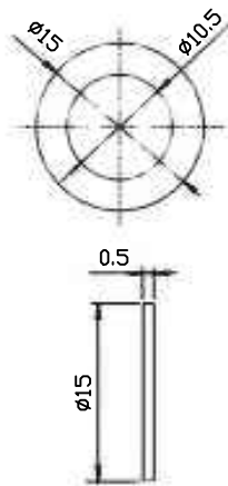
FLAT WASHER
