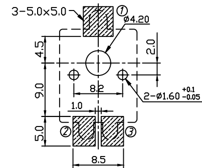
PCB Layout ±0.1 Solder Pad
