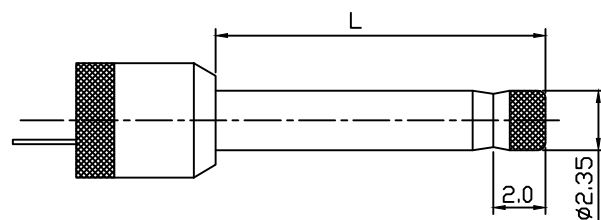
RECOMMENDED PLUG
