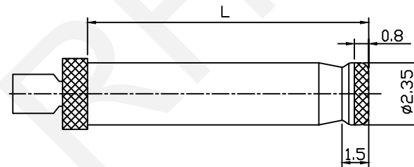
RECOMMENDED PLUG
