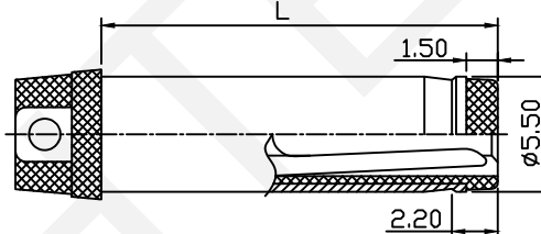
RECOMMENDED PLUG
