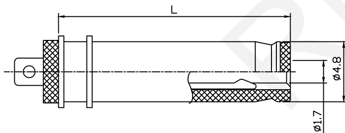
RECOMMENDED PLUG
