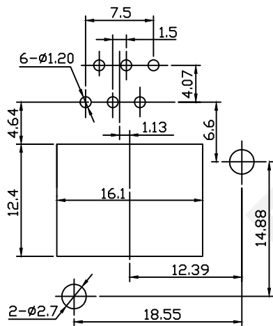
PCB Layout
