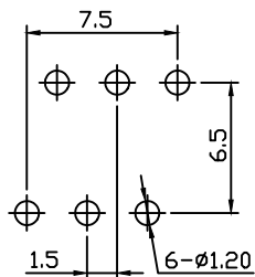
PCB Layout
