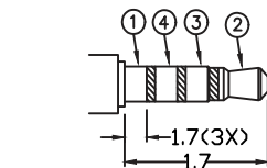
Ø2.5 SPECIAL MATE PLUG
