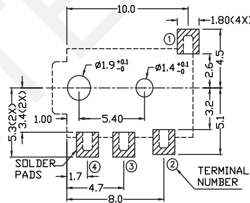
RECOMMENDED SOLDER PAD LAYOUT (TOP VIEW)
