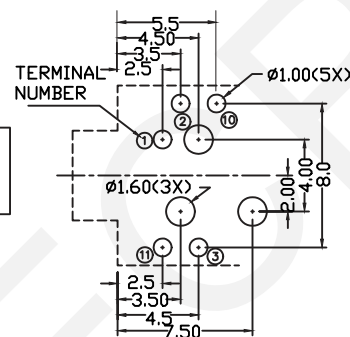
PCB LAYDUT <BOTTOM VIEW>
