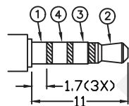
Ø2.5 SPECIAL MATE PLUG
