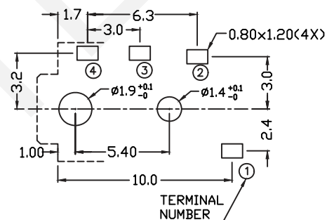
PCB LAYOUT (BOTTOM MEW)
